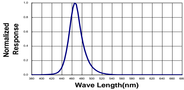
Spectral Radiance (Peak @ 468nm)
